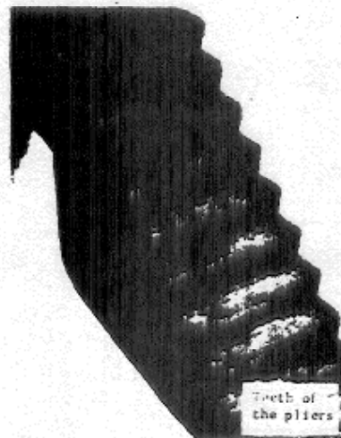
FIG. 14—The striations caused by using the tool are 90 deg from the direction of the potential repetitive structural characteristics that would be produced, if possible, by the broaching tool. The photograph shows one of the as-broached jaws.
