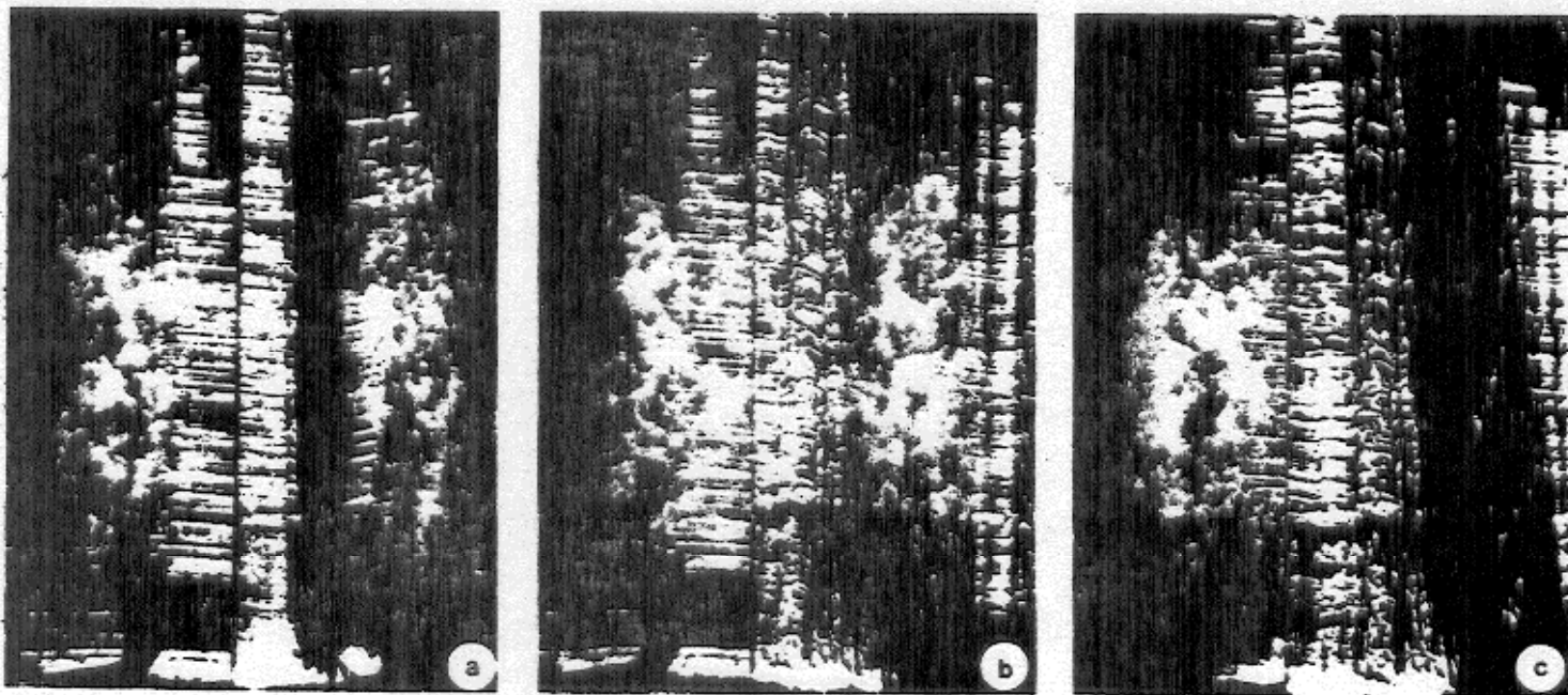
FIG. 11—Photomicrographs of toolmark striations from the as-broached jaws showing individuality of specific teeth: (a) Pliers 1 and 2, (b) Pliers 1 and 3, and (c) Pliers 2 and 3.
