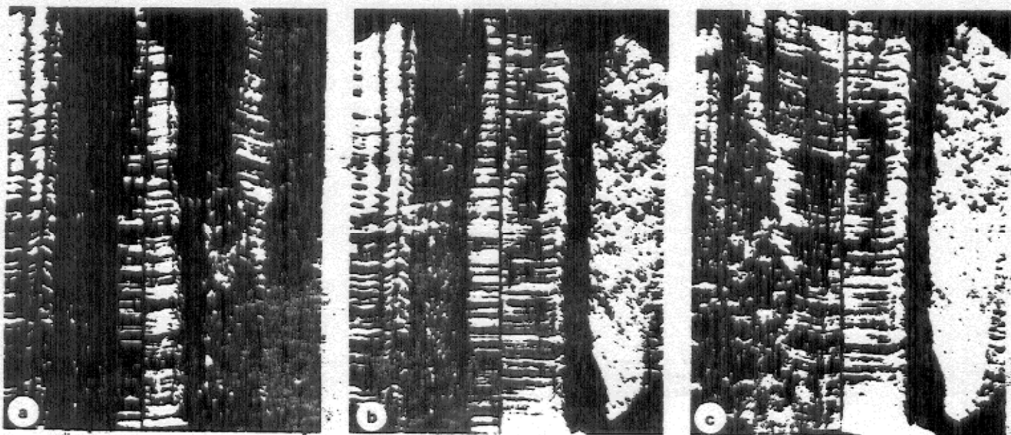
FIG. 12—Photomicrographs of toolmark striations from the chromium-plated jaws showing individuality of specific teeth: (a) Pliers 1 and 2, (b) Pliers 1 and 3, and (c) Pliers 2 and 3.
