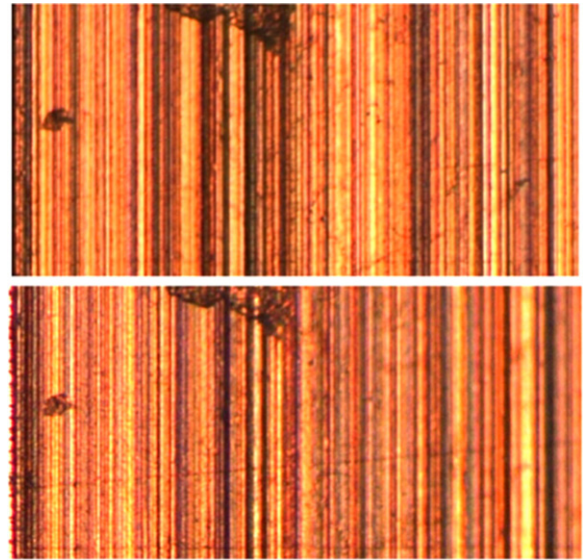
Figure 2. Two images captured on the same area of the SRM 2460-001 bullet by the same microscope under different lighting directions. Top—area aligned perpendicular to microscope optical axis, bottom—the same area tilted by approximately 6°.
